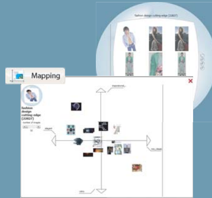
Mapping generation
